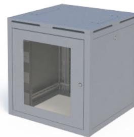
15U 780 x 780 Height: 815mm
