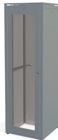
39U 600 x 600 Height: 1881mm
