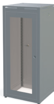
27U 600 x 600 Height: 1348mm
